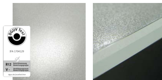
Non-slip class R12 full-surface etching
