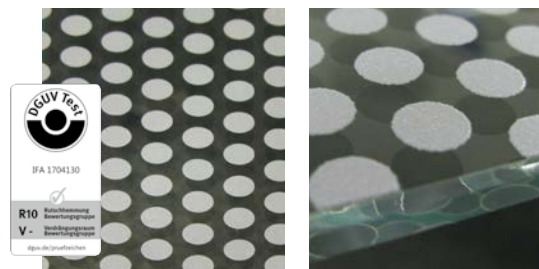
Non-slip class R10 in dot pattern; print area 40 %, 8 mm dots
